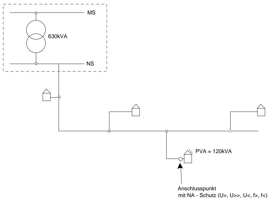
Trafostation (NE6)
